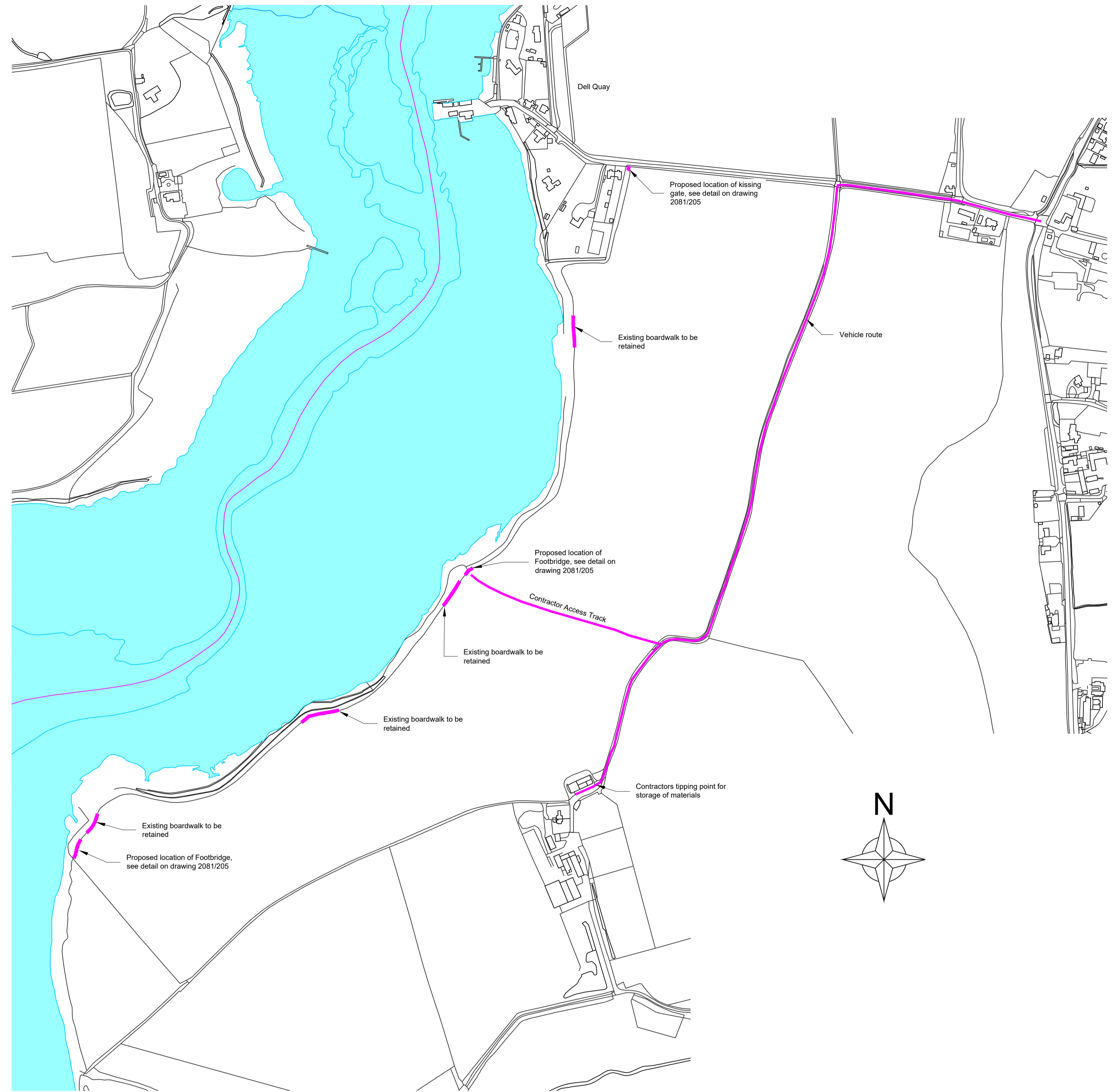
Site Plan 1:4000 SCALE BAR FOR ALL 1:4000 DETAILS 0m 100m 200m 300m 400m
